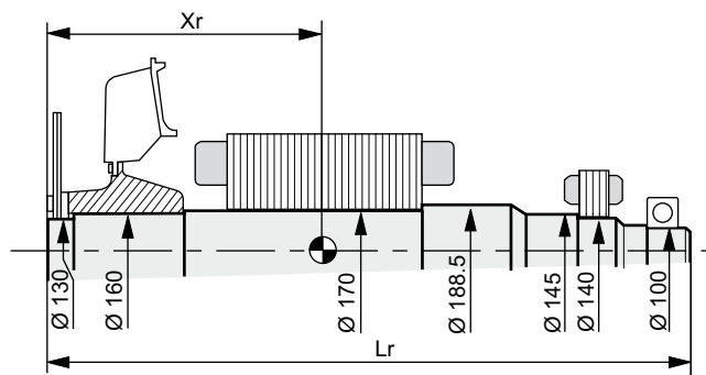
Centre of gravity : Xr (mm), rotor length Lr (mm), Weight : M (kg), Moment of inertia : J (kgm 2 ) : (4J = MD 2 )
